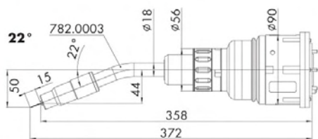
Dimensional sketch ABIROB® W (incl. robot flange)
