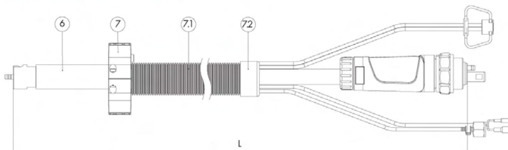
Cable assembly liquid-cooled for iCAT
