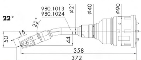
Dimensional sketch ABIROB® A (incl. robot flange)
